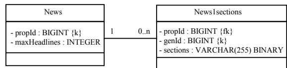
Figure 8. Tables (MySQL) generated for the meta-information specified in Figure 7.
