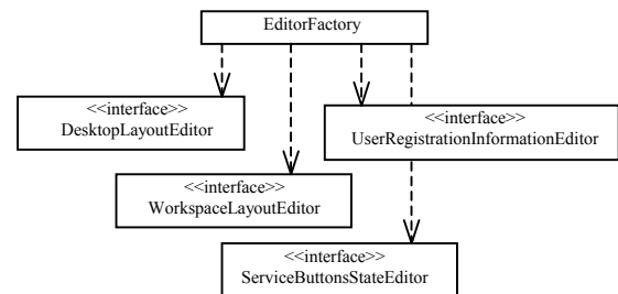
Figure 12. Editors for personal persistent objects.
