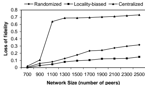
Figure 2: Performance Evaluation
