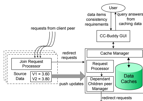
Figure 1: CC-Buddy System Architecture
